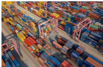
KALMAR 26 SWL 40 tons E.RTG 5 + 1 Tier 6 + 1 Row Sunitomo MES
